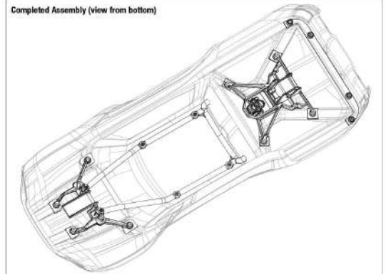
Completed Assembly (view from bottom)
