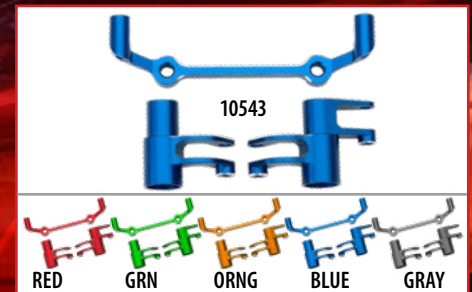
Steering Bellcranks & Drag Link, 6061-T6 aluminum, five available colors
